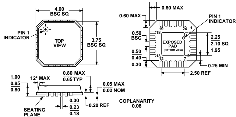
Figure 34. 24-Lead Lead Frame Chip Scale Package [LFCSP] 4 mm x 4 mm Body (CP-24-1) Dimensions shown in millimeters
